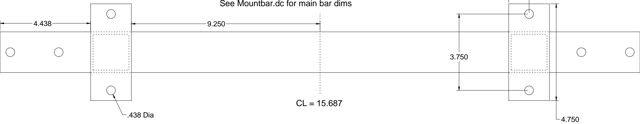
Flathead Front Engine Mount Bar (mountbarflatheadfront.dc)
