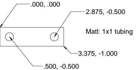
Generic Engine Mount Bar (mountbar.dc)
