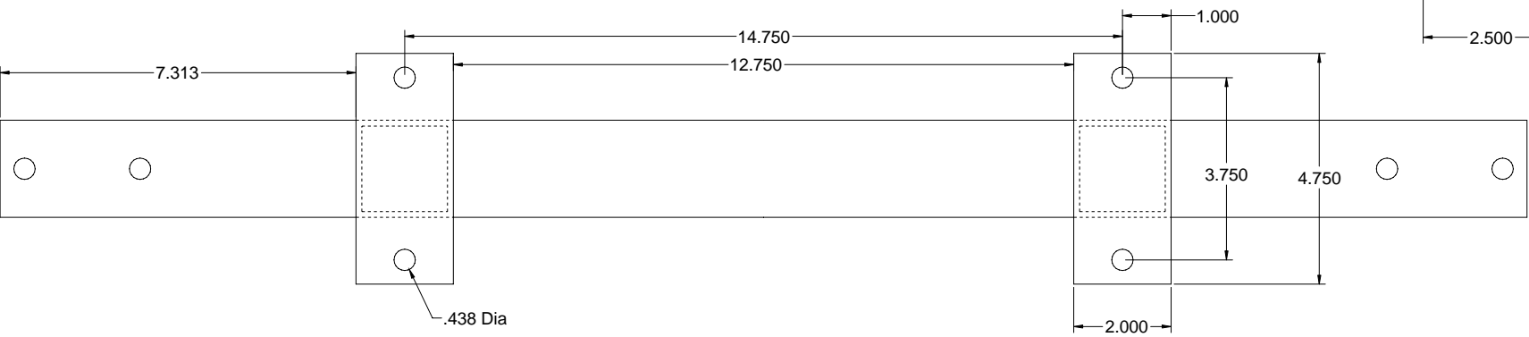
Small Block Ford Front Engine Mount Bar (mountbarSBFfront.dc)
