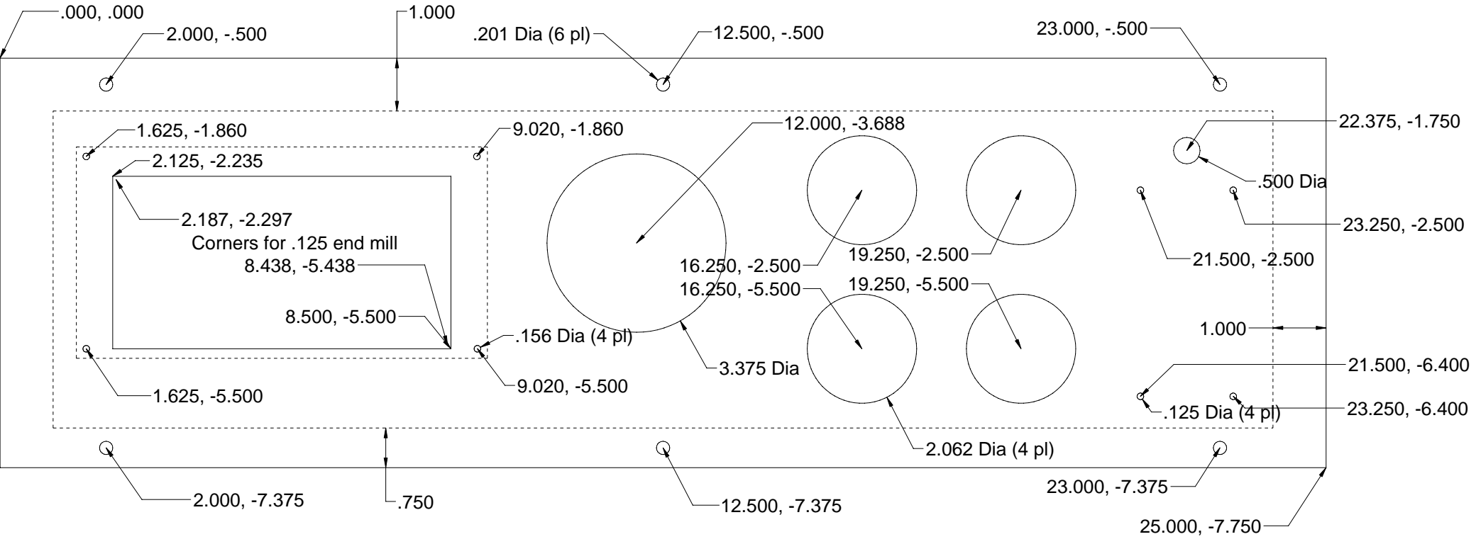
MountBarDashPanel
